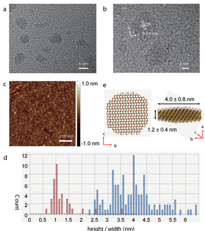
Figure 1. a,b) TEM images of TGA-stabilized \text{FeS}_2 NPs. The crystalline lattice of the bc plane can be seen. c) AFM image of TGA-stabilized NPs deposited on a silicon wafer. d) The statistical distribution of NP heights (red) and diameters (blue) determined from AFM and TEM images, respectively. e) Model atomic structure of the discoid \text{FeS}_2 NP. TGA stabilizers are omitted for clarity. The brown and yellow junctions indicate iron and sulfur atoms, respectively.
